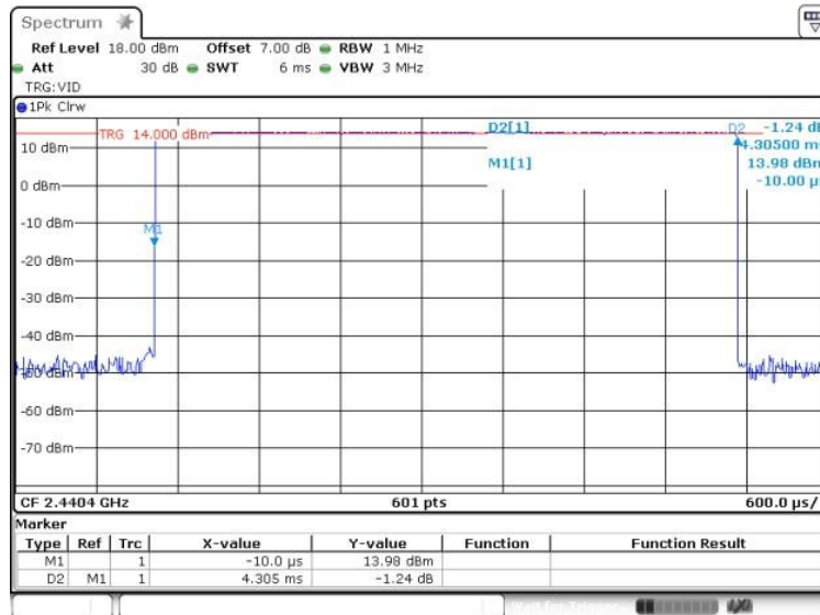
GFSK on time/100 ms (One Pulse) Plot on Channel 49
