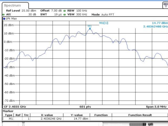
GFSK LOW CHANNEL, CARRIER LEVEL
