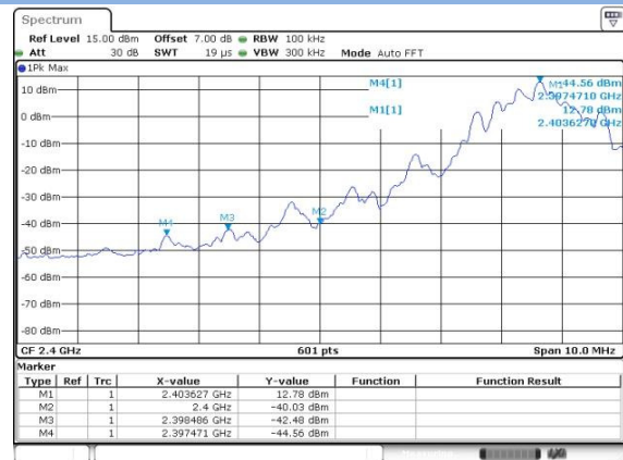
GFSK LOW CHANNEL, BAND EDGE
