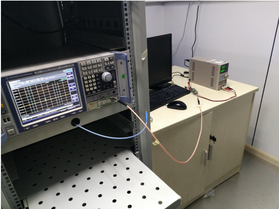
Conducted Test
