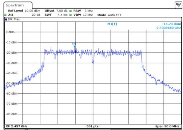
802.11g MIDDLE CHANNEL
