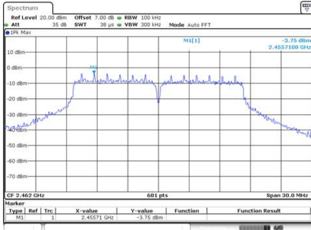
802.11g HIGH CHANNEL, Carrier level
