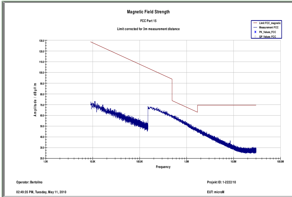
Plot 1: TX mode, 9 kHz – 30 MHz
