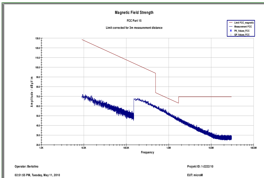
Plot 2: RX mode, 9 kHz – 30 MHz
