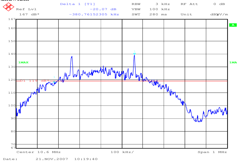
Plot 3 20 dB-Bandwidth
