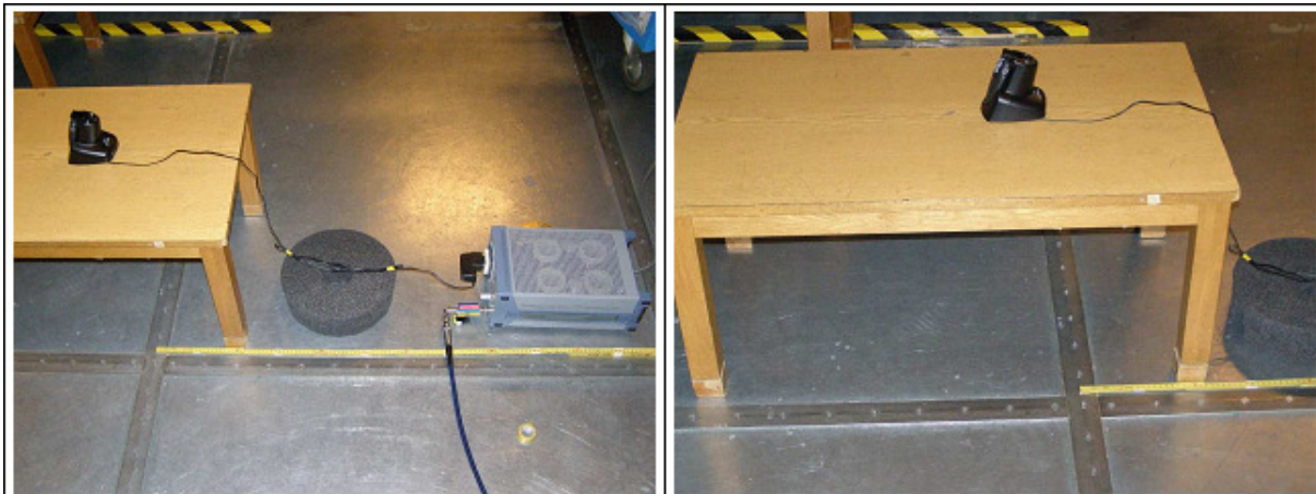
Conducted Emission – interference voltage
