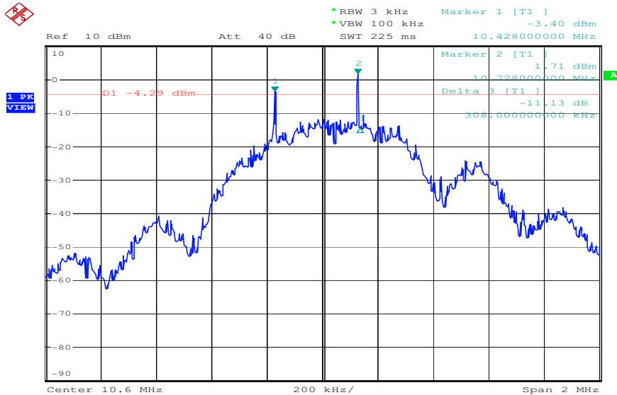
Plot 1: 6 dB-Bandwidth
