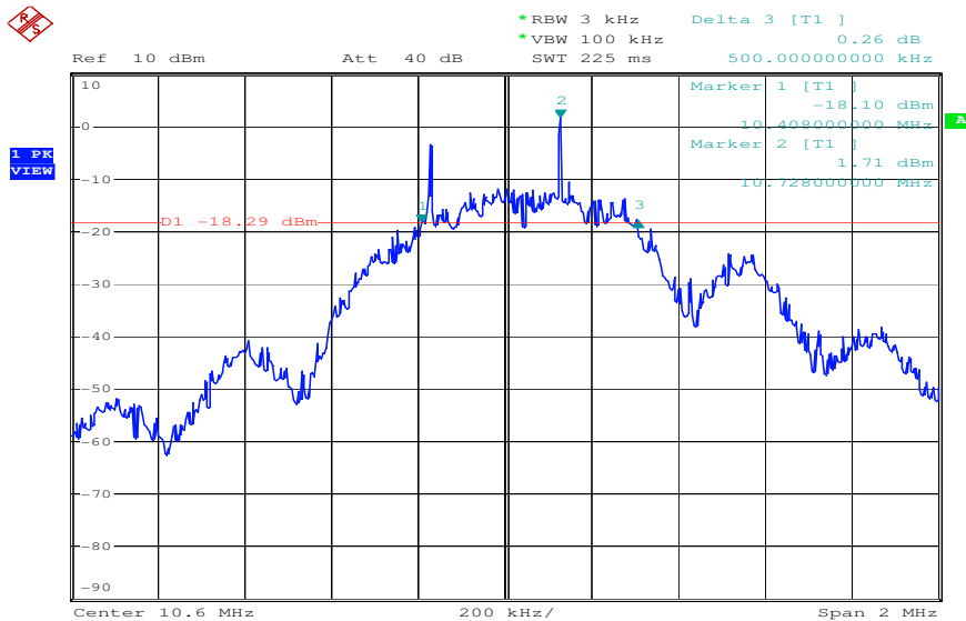
Plot 2: 20 dB-Bandwidth
