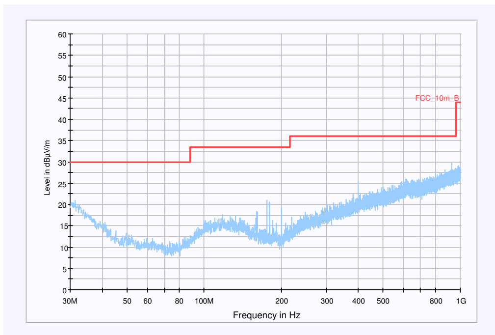
Plot: 0.03 - 1 GHz vertical/horizontal (highest channel)
