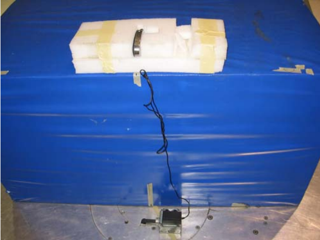
Antenna Conducted Emissions Setup
