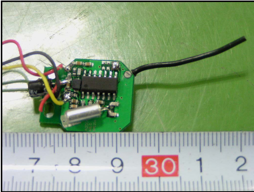
EUT – RF Board Top Components View
