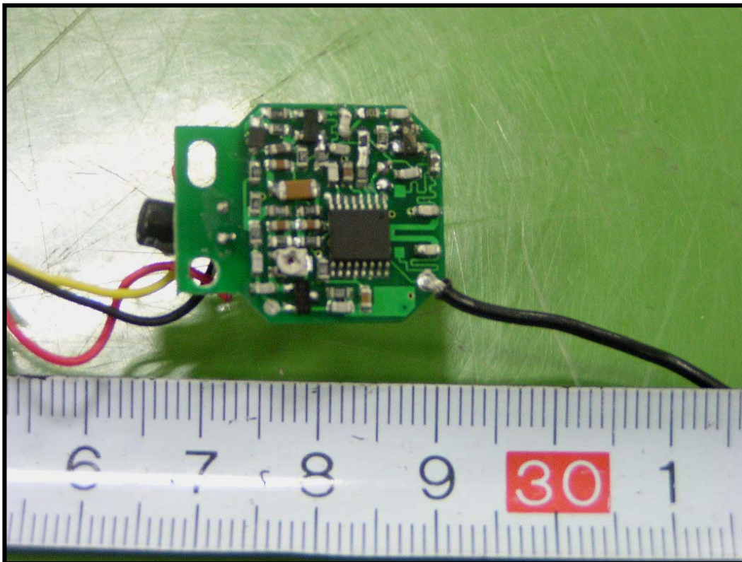
EUT – RF Board Bottom Components View
