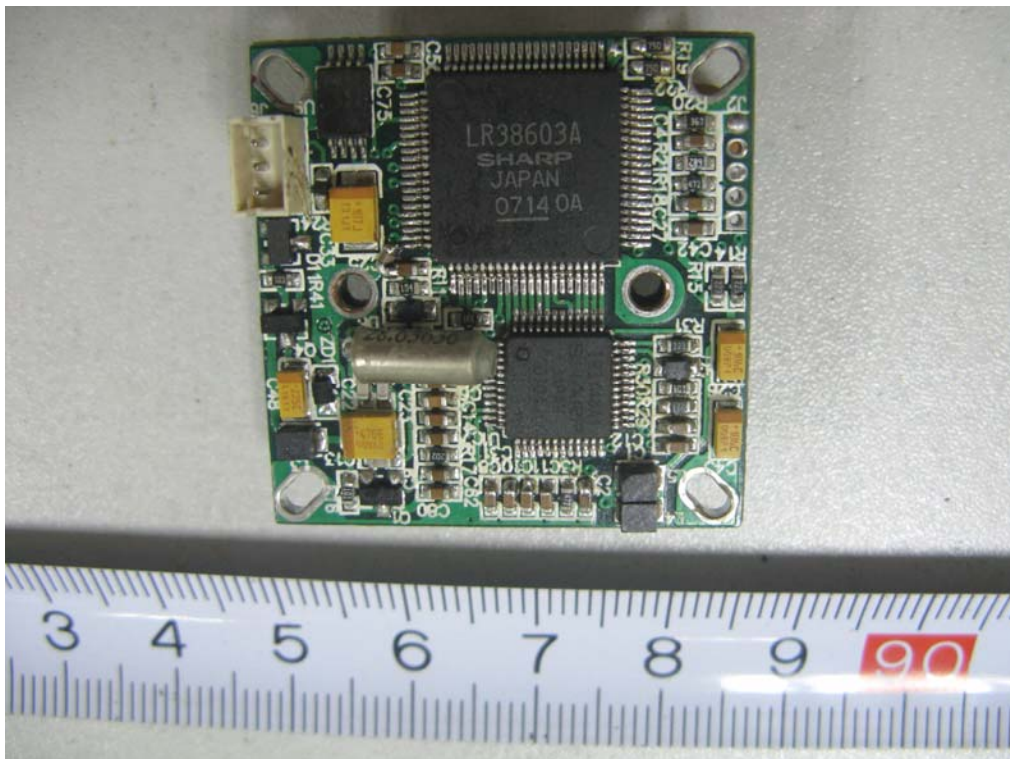
EUT – Camera Board Bottom Components View
