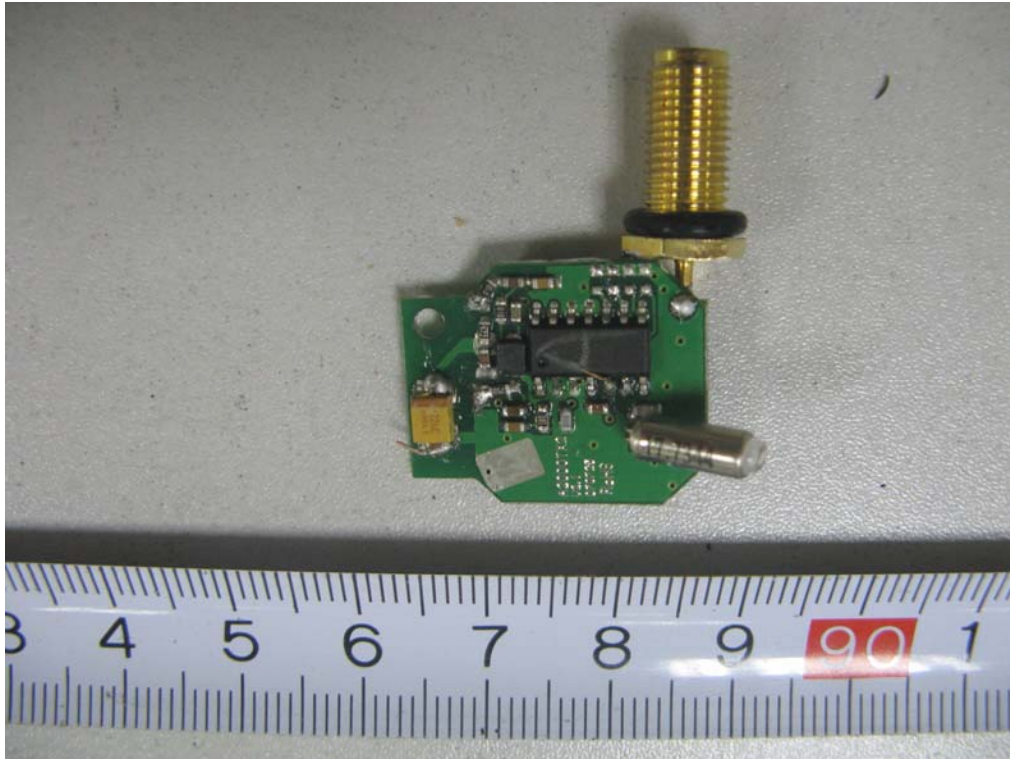
EUT – RF Board Top Components View
