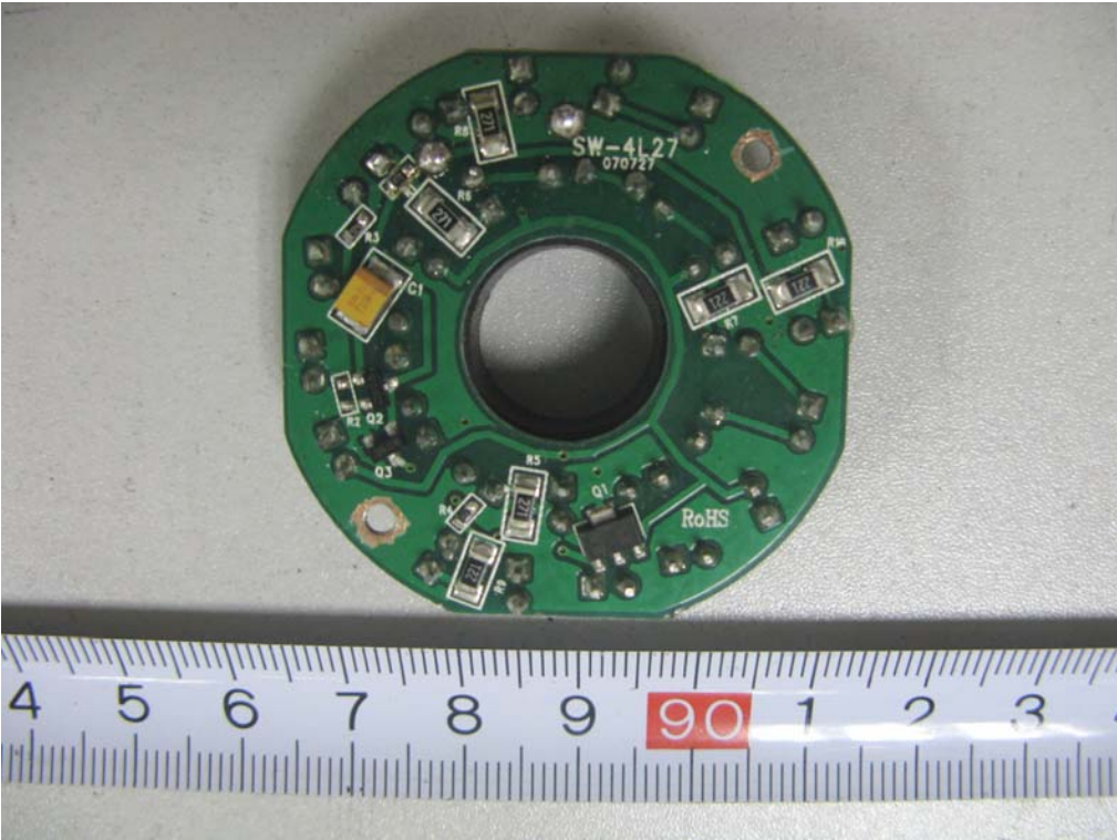
EUT – LED Board Bottom Components View
