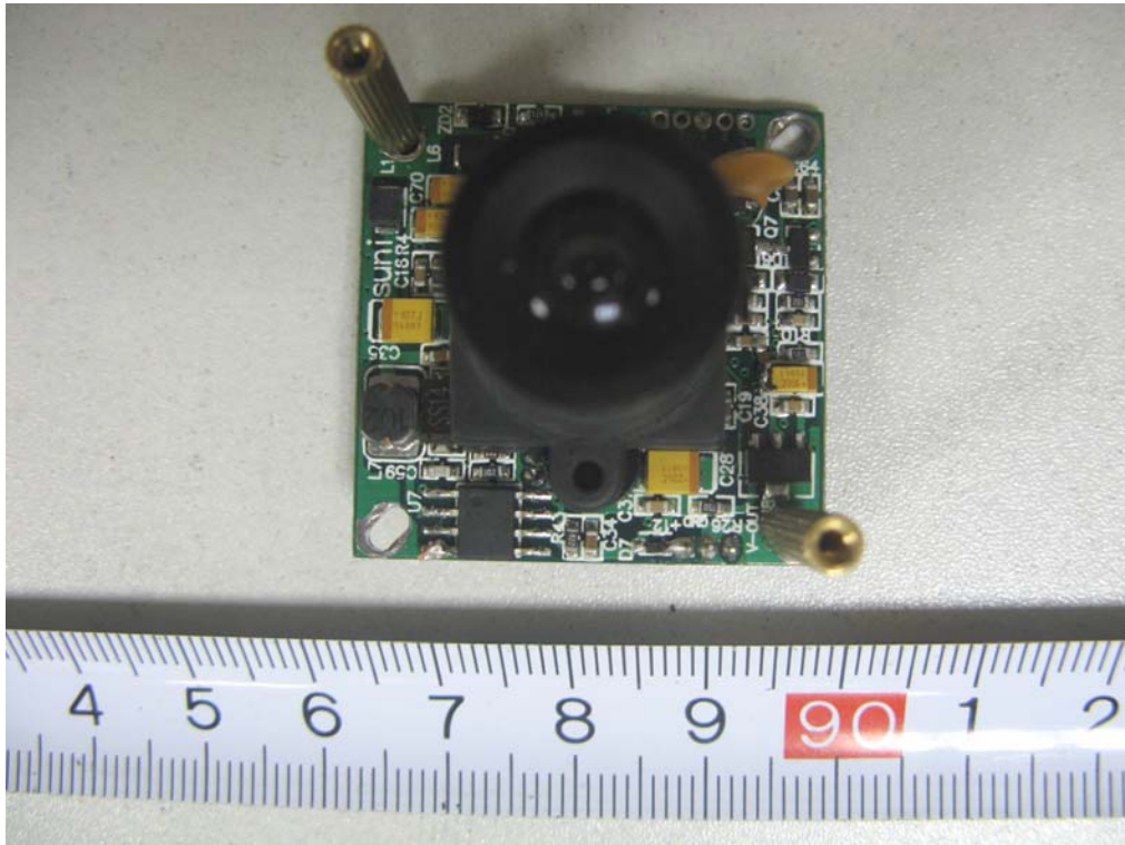
EUT – Camera Board Top Components View
