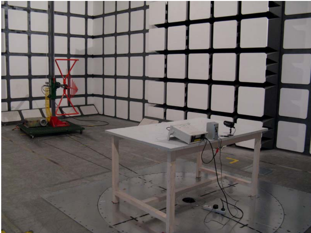
Radiated Emissions - Rear View (30 MHz-1 GHz)
