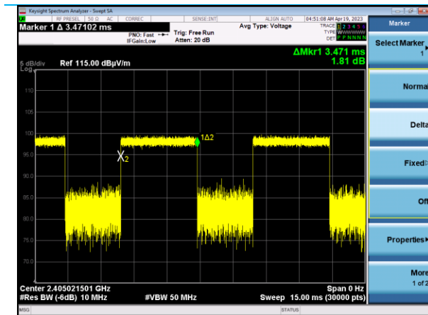
On Time 3.471ms
