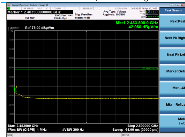
2.4835-2.5 GHz Vertical EUT Horizontal, Ch 16 Average
