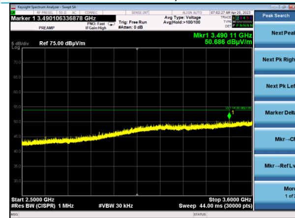
2.5-3.6 GHz Horizontal EUT Horizontal, Tx Mid
