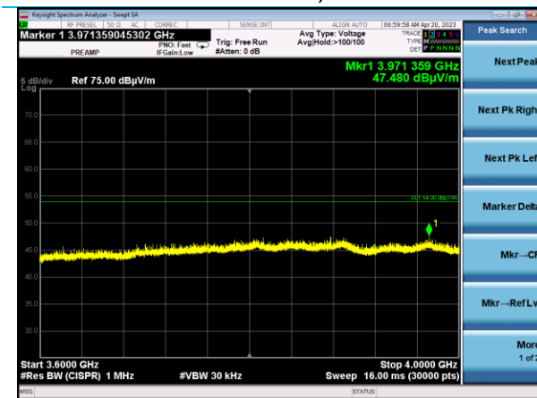
3.6-4 GHz Horizontal EUT Horizontal, Tx Mid
