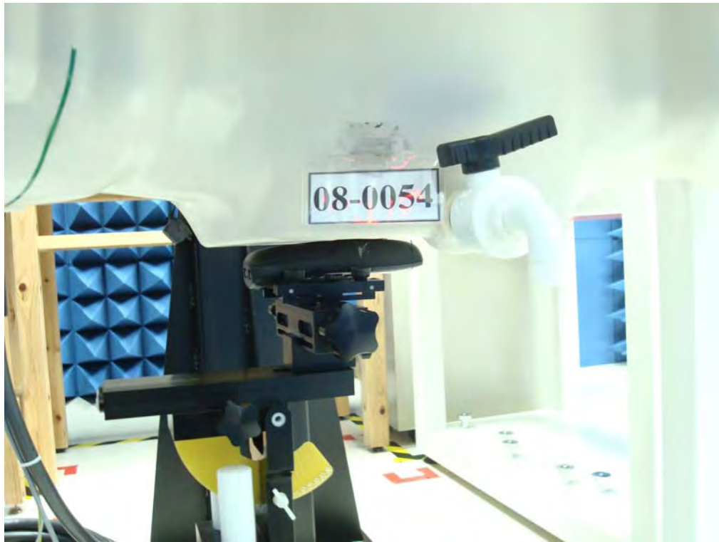
Figure 17. Body SAR Test Setup_ (Flat Section)
