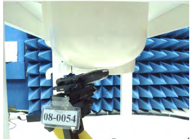
Figure 16.Left Head SAR Test Setup (Tilted)
