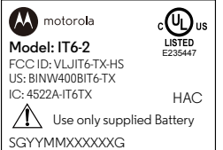
Handset Label Handset label size: W 32mm x H 23mm
