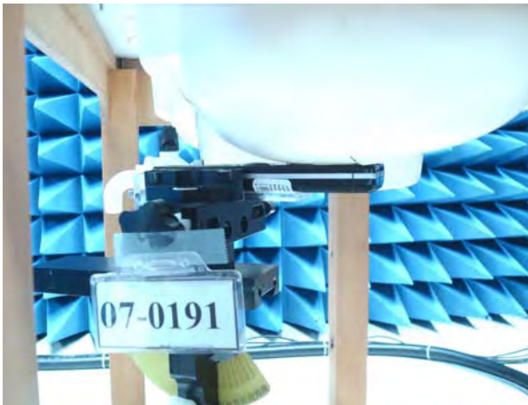
Figure 15. Left Head SAR Test Setup (Cheek)
