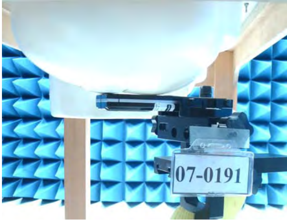
Figure 13. Right Head SAR Test Setup (Cheek)
