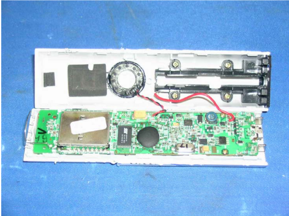
Handset assembly
