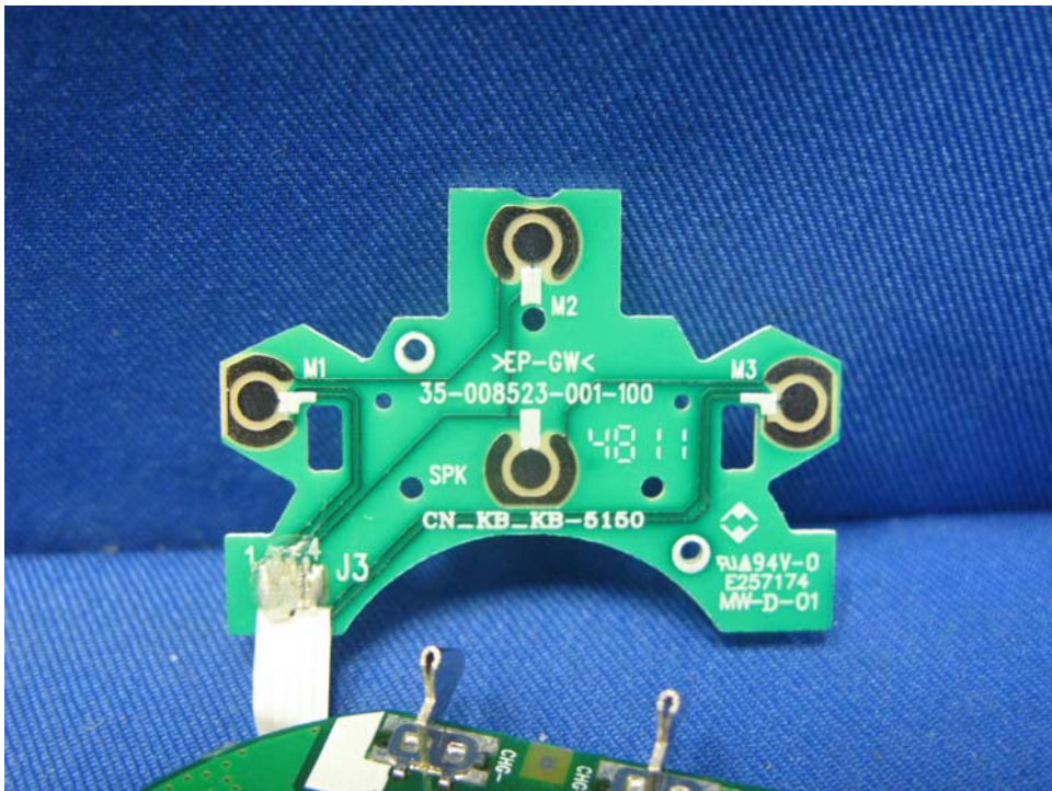
Speaker Pad Keypad front side
