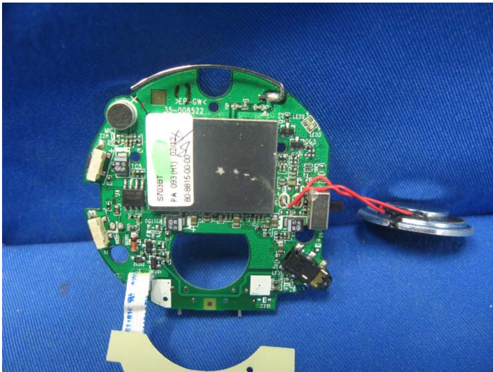
Speaker Pad Main PCB comp side
