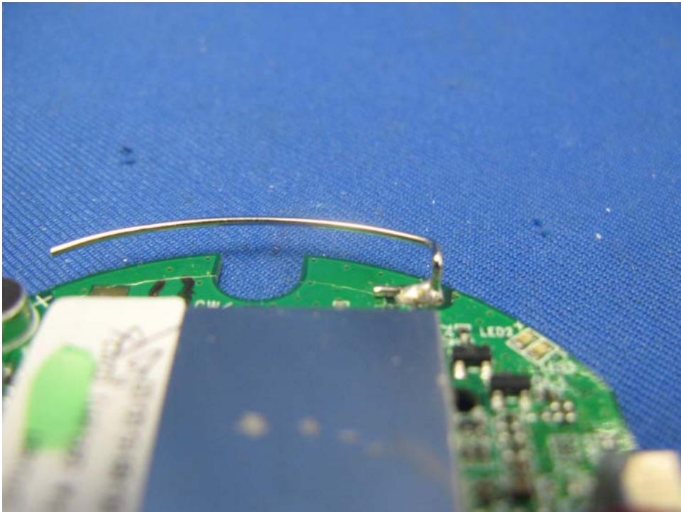
Speaker Pad Antenna
