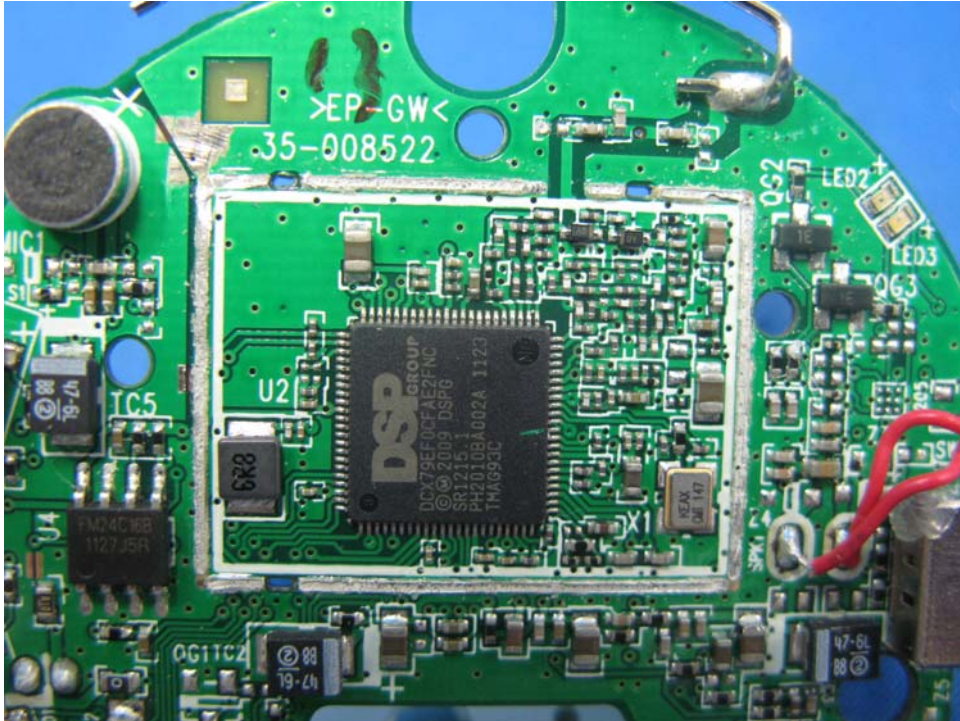
Speaker Pad Oscillator PCB comp side
