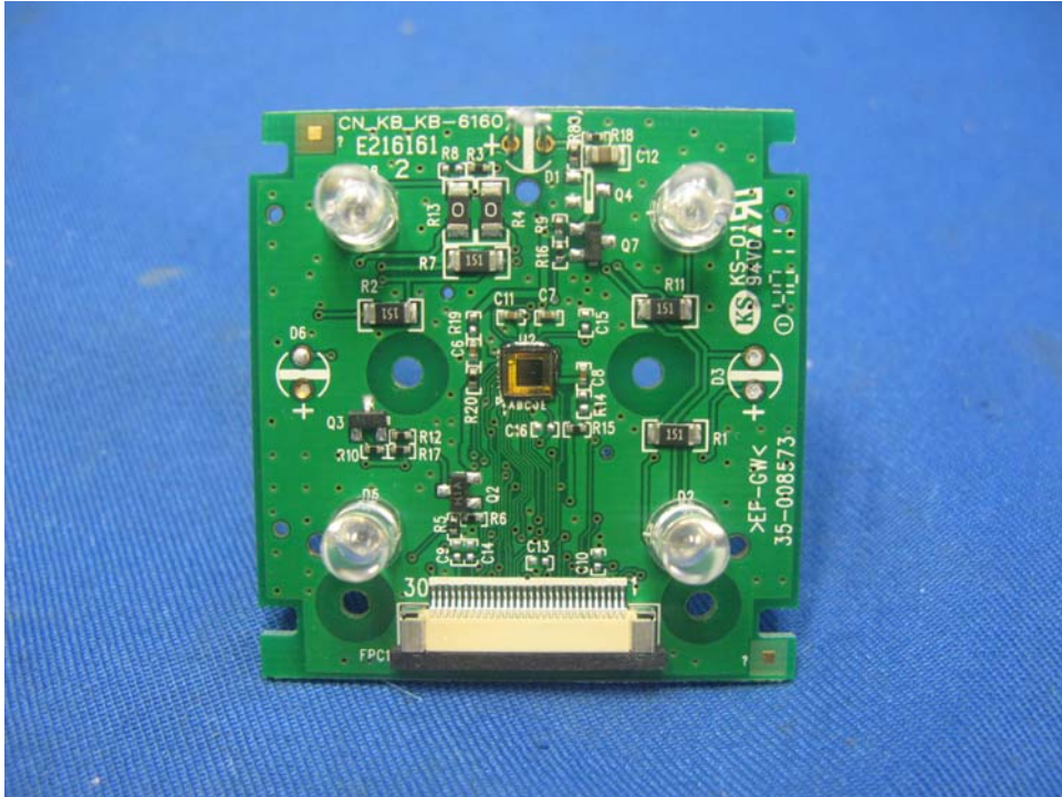
Baby Unit Camera PCB front side
