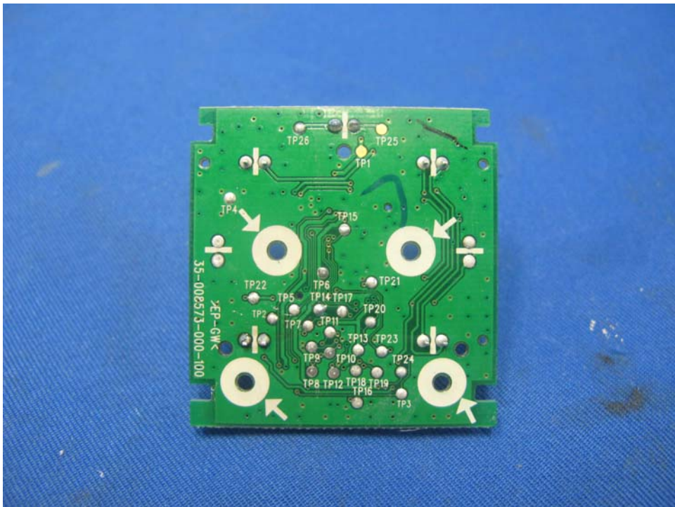
Baby Unit Camera PCB rear side
