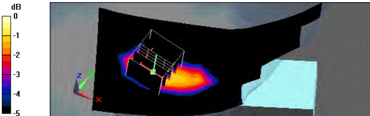
0 dB = 0.018mW/g
