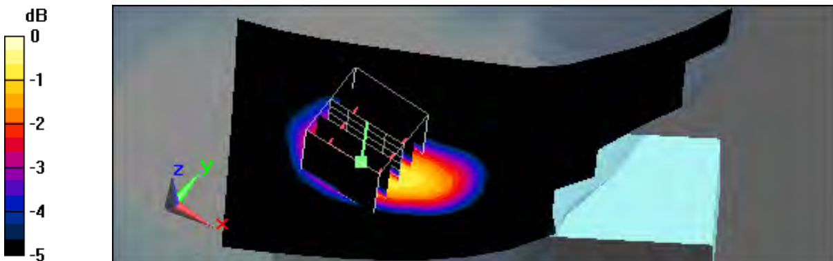
0 dB = 0.021mW/g
