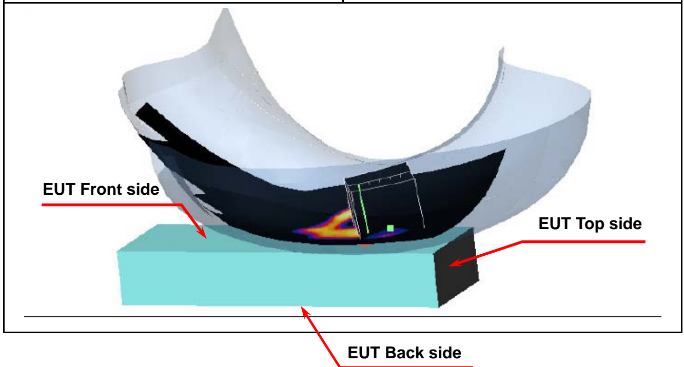
Figure 4. Left Head SAR Test Setup (Cheek)
