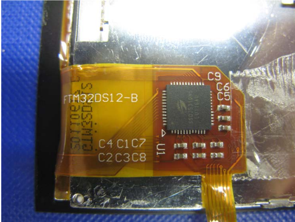
Handset LCD View 2
