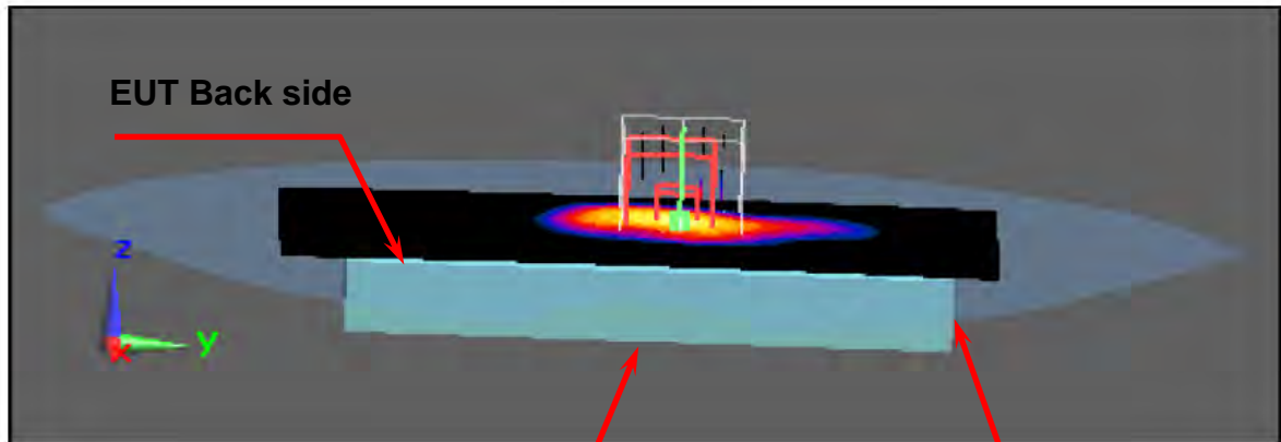
Figure 7. Body SAR Test Setup (Flat Section)
