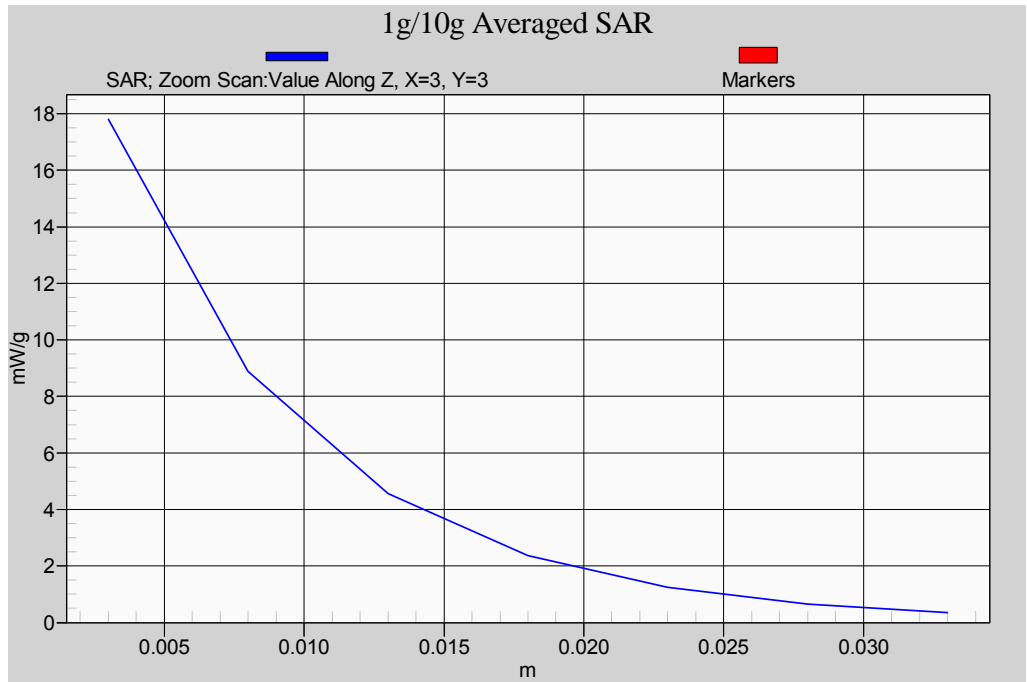
Head-Tissue-Simulating-Liquid 2450MHz
