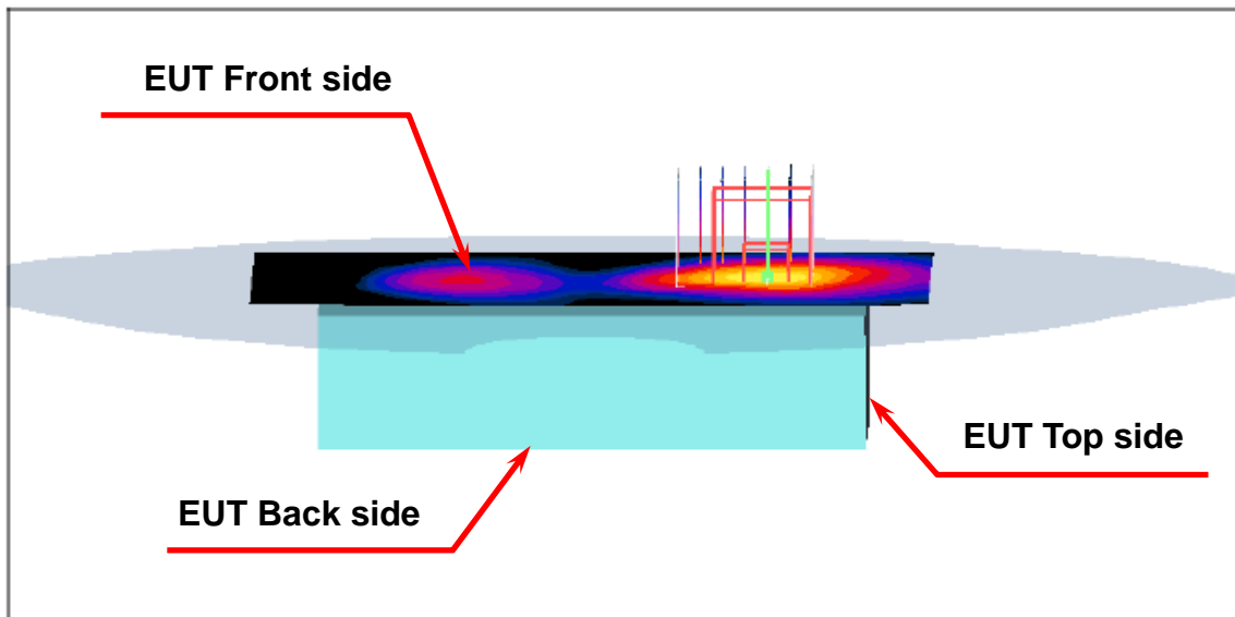
Figure 2. Body SAR Test Setup (Flat Section)
