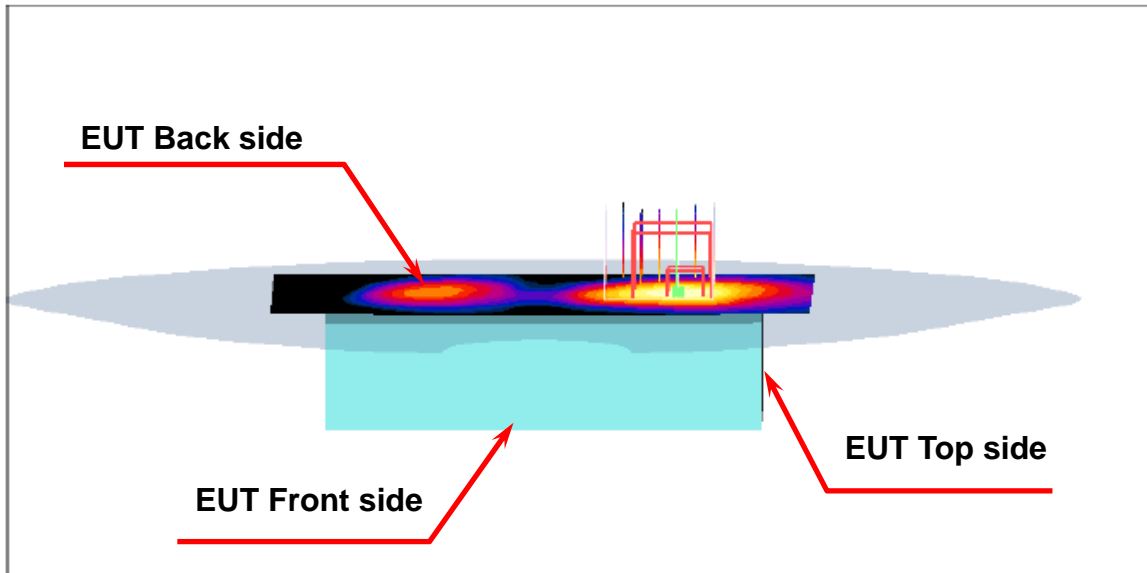
Figure 4. Body SAR Test Setup (Flat Section)
