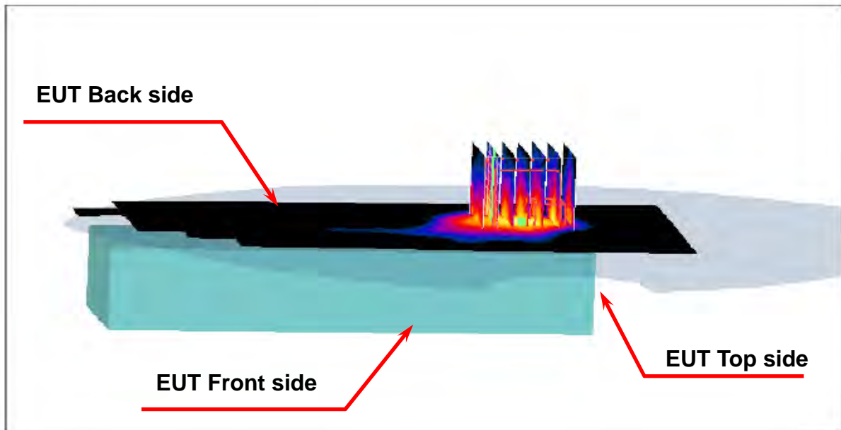
Figure 7. Body SAR Test Setup (Flat Section)
