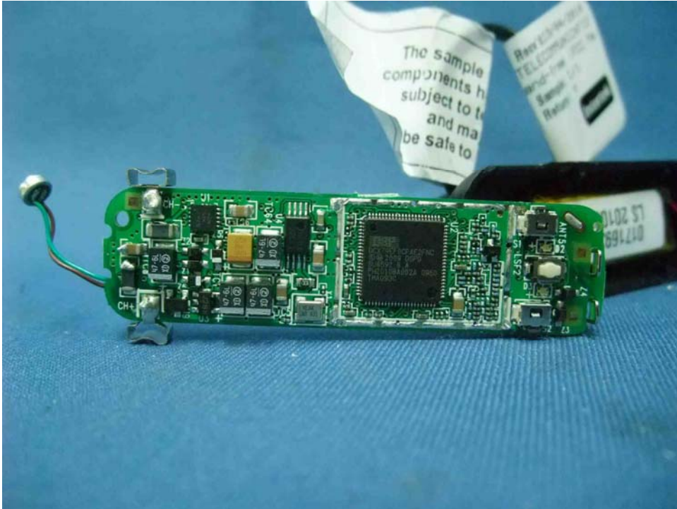
Headset Main PCB comp side (View 2)
