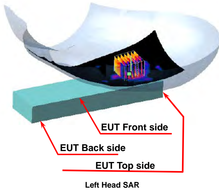
Figure 4. Left Head SAR Test Setup (Cheek)
