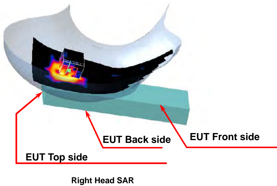
Figure 2. Right Head SAR Test Setup (Cheek)
