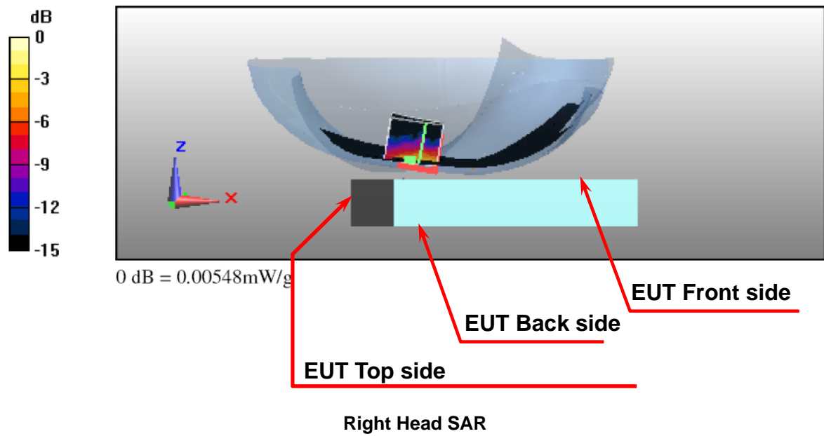
Figure 2. Right Head SAR Test Setup (Cheek)
