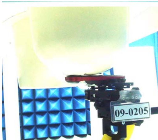
Figure 2. Right Head SAR Test Setup (Cheek)
