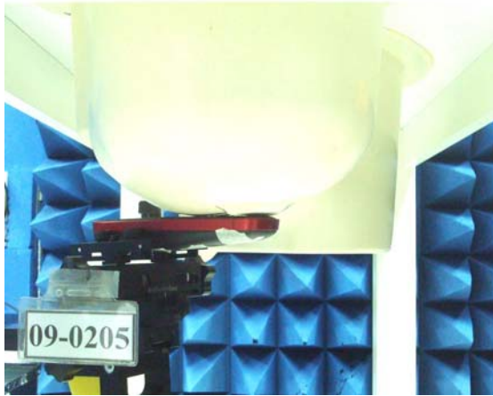
Figure 4. Left Head SAR Test Setup (Cheek)
