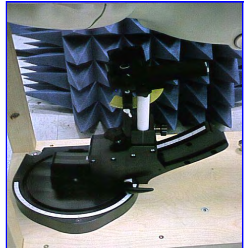
Figure 9. Device Holder
