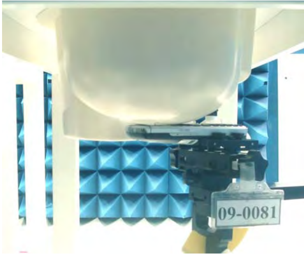
Figure 14. Right Head SAR Test Setup (Cheek)
