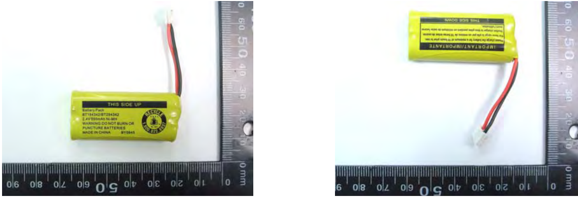
Figure 2. Battery (Ni-MH 2.4V , 550mAh)
