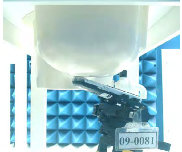
Figure 15. Right Head SAR Test Setup (Tilted)
