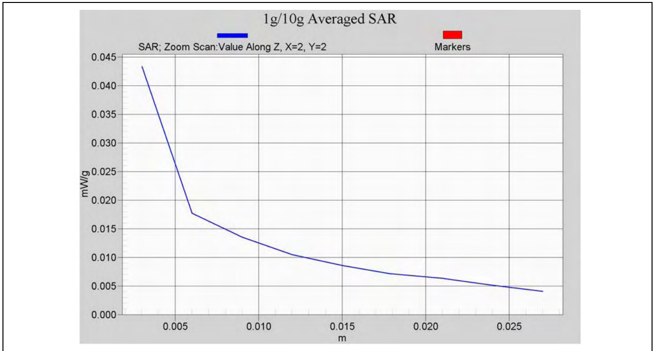
Body SAR Measurement _ Back to Phantom 2mm separation _ CH2
