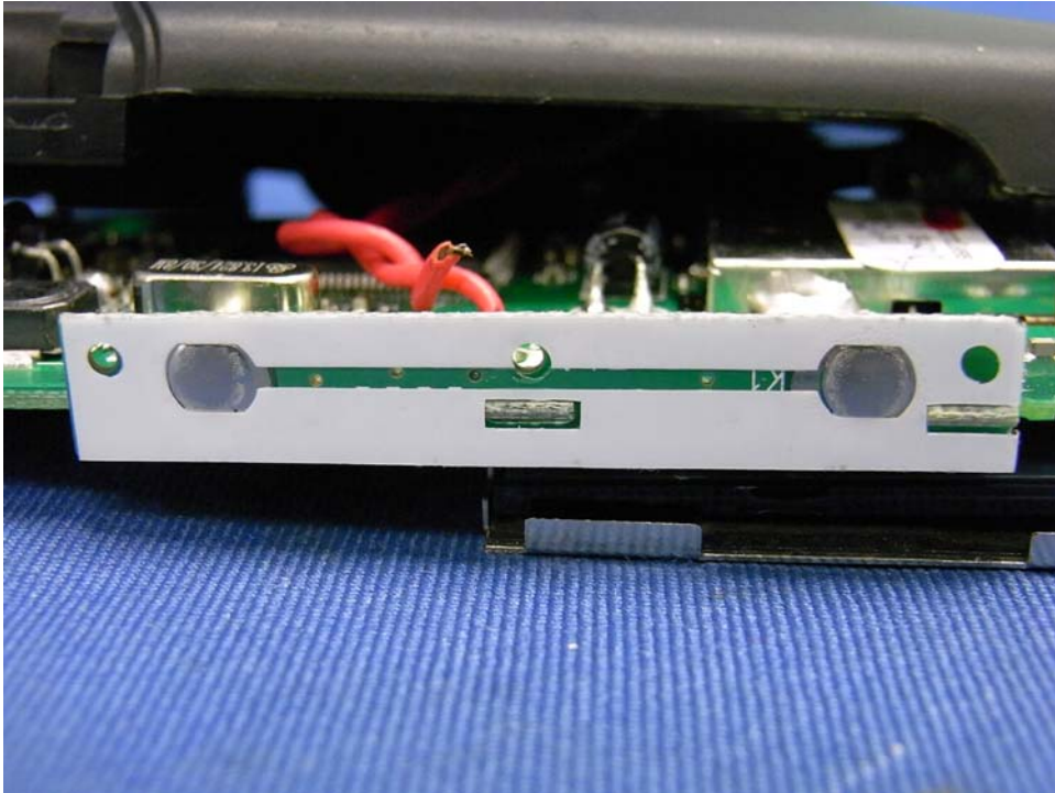
Handset Main PCB display side (View 5)
