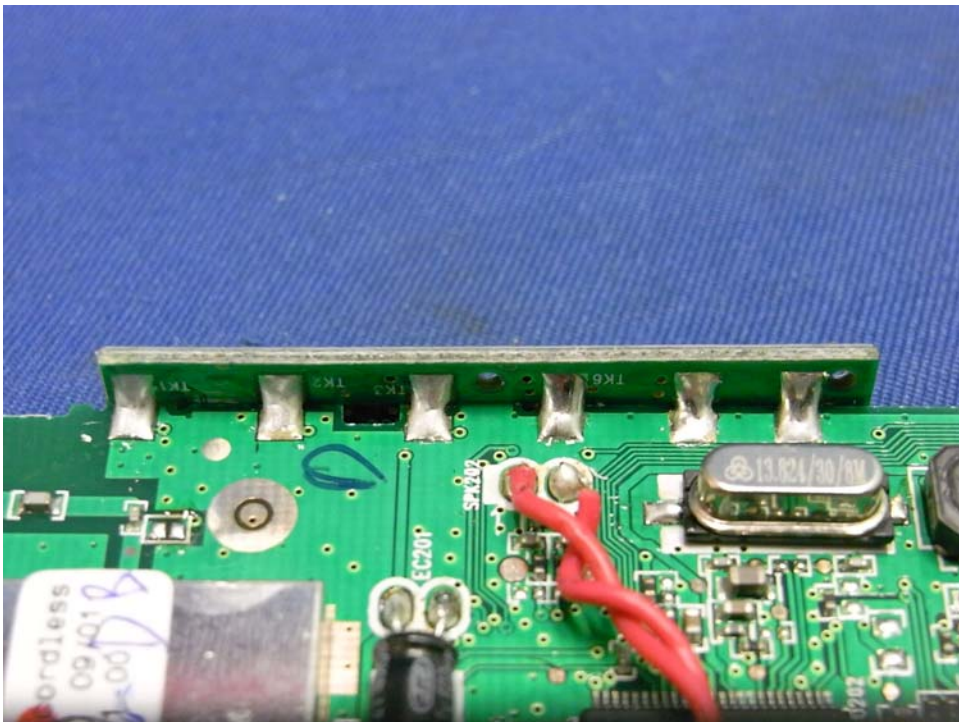
Handset Main PCB display side (View 6)
