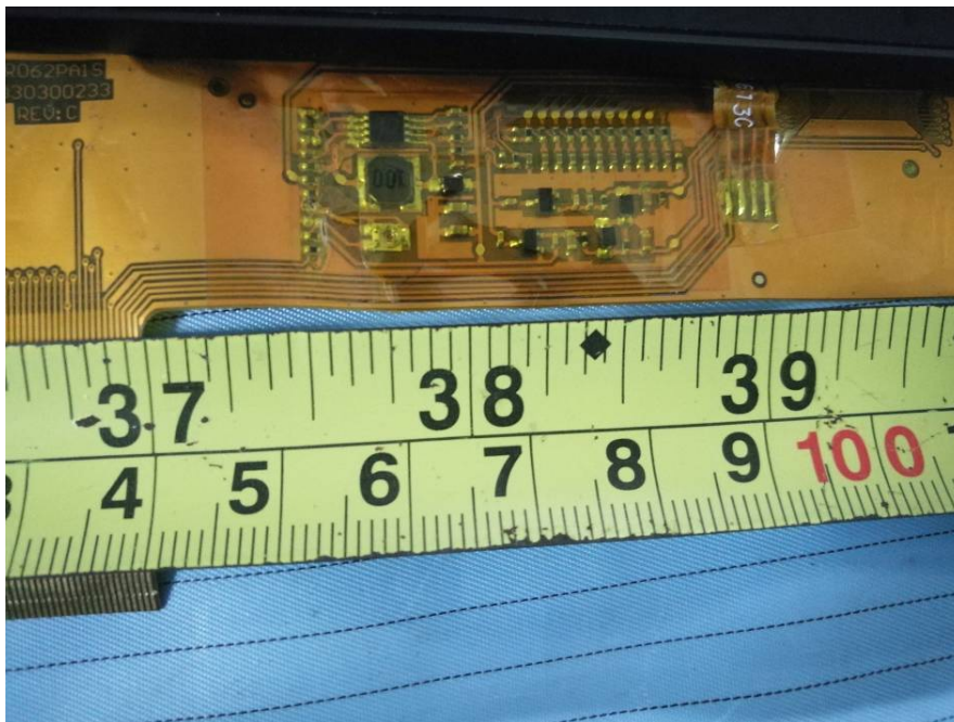
EUT – FPC Softly Board View
