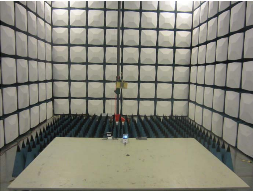
Radiated Emission - Rear View (Charging Adapter 1) (Above 1GHz)
