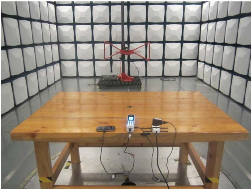
Radiated Emission - Rear View (Charging Adapter 1) (Below 1GHz)
