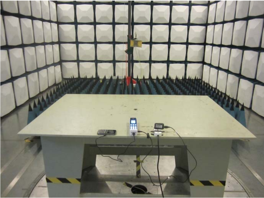
Radiated Emission - Rear View (Charging Adapter 2) (Above 1GHz)
