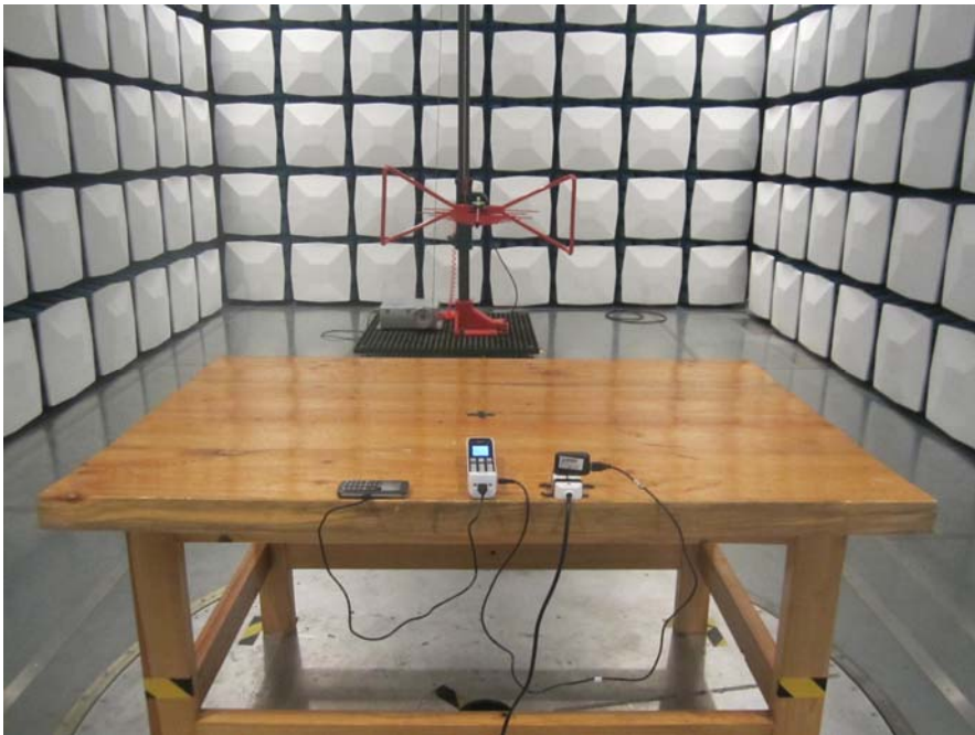
Radiated Emission - Rear View (Charging Adapter 2) (Below 1GHz)
