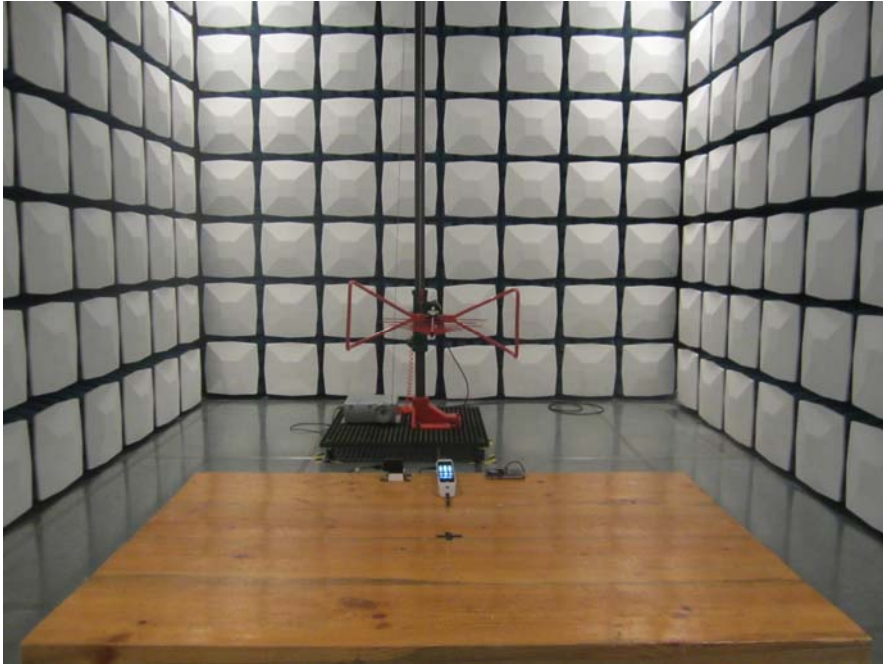
Radiated Emission -Front View (Charging Adapter 2) (Below 1GHz)
