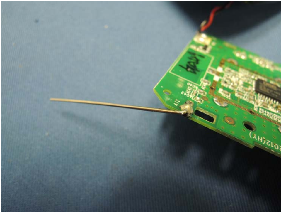
Handset Antenna
