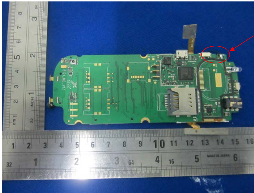
EUT –Main Board Bottom Speaker Shielding Off View
