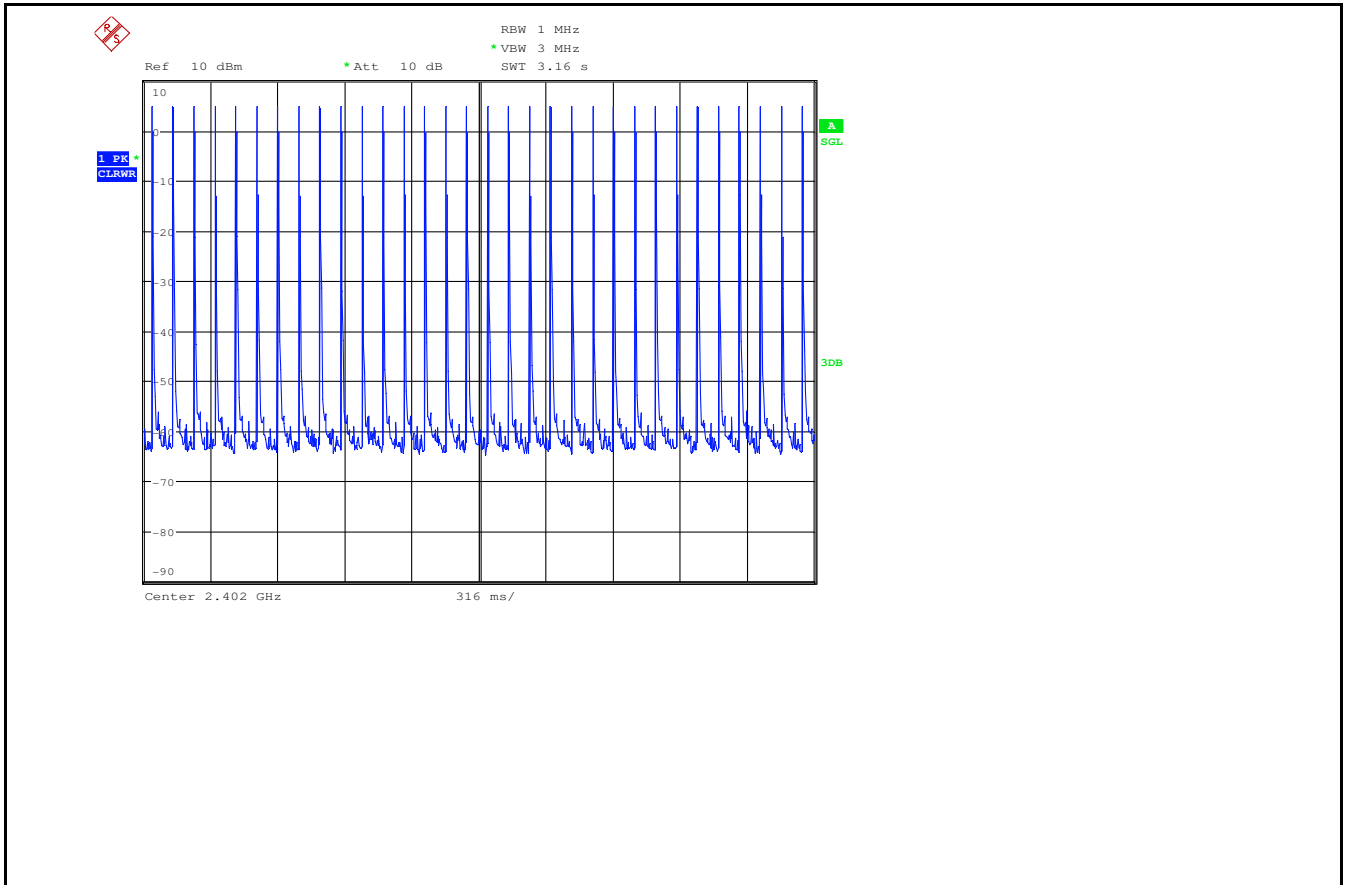
Dwell Time_3DH3_2402
