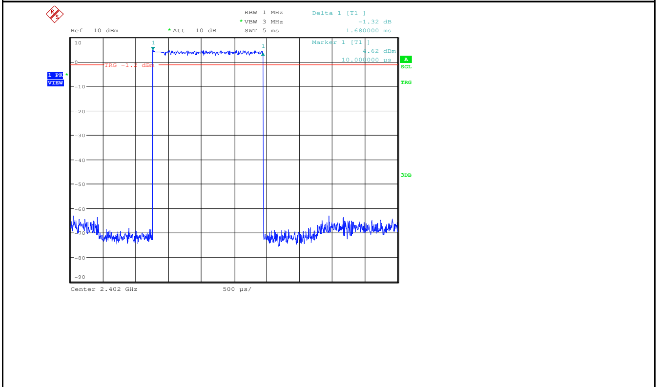
Dwell Time_3DH3_2402
