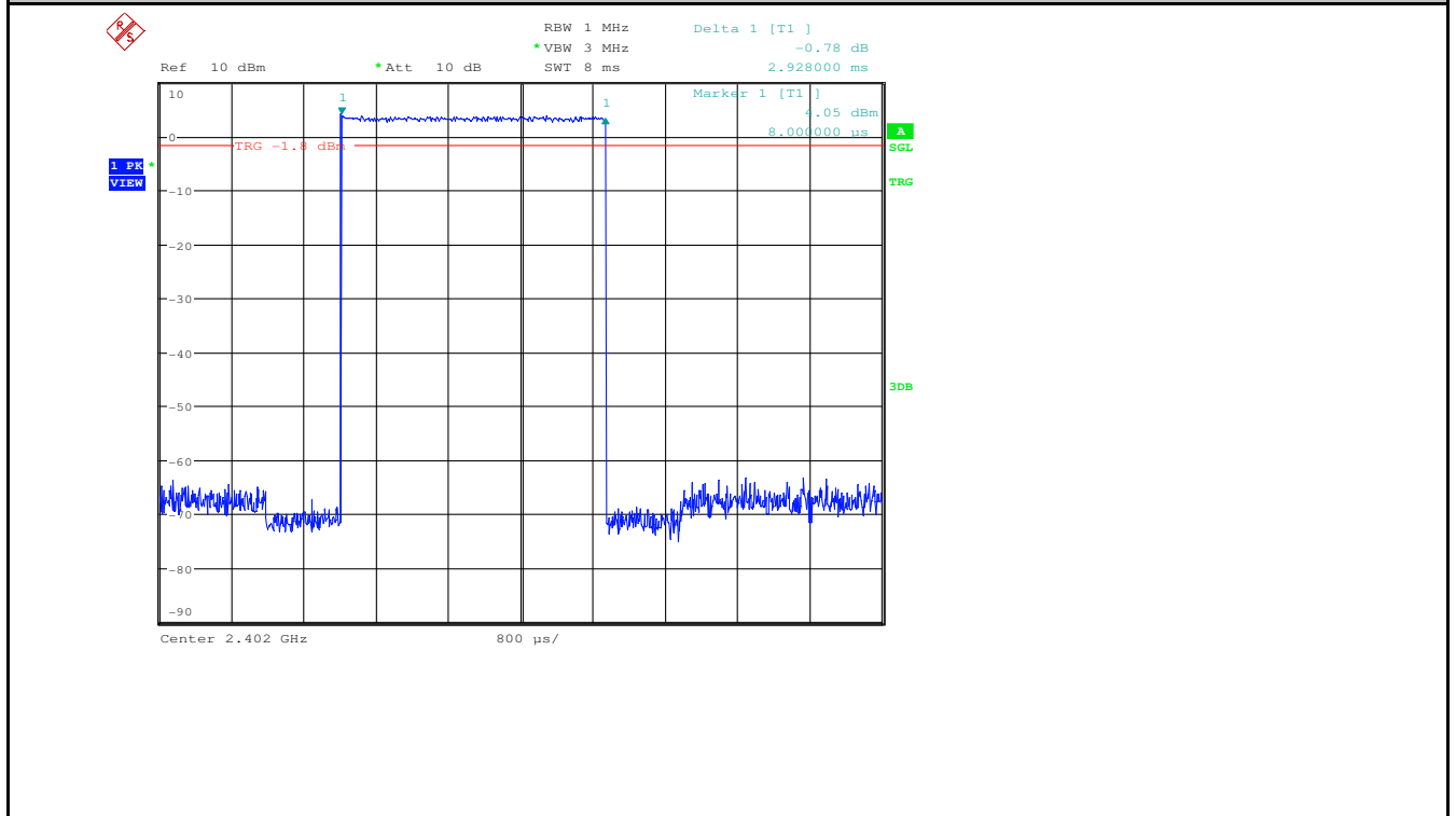
Dwell Time_2DH5_2402
