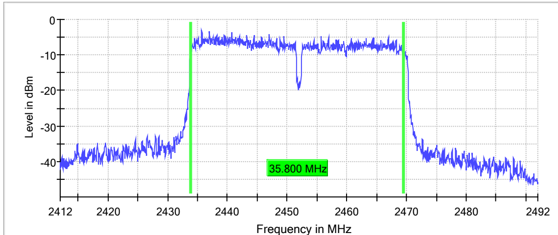
6 dB Bandwidth
