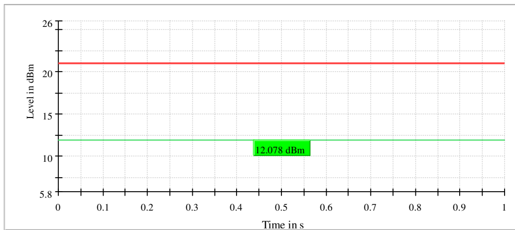
Gated Trace
