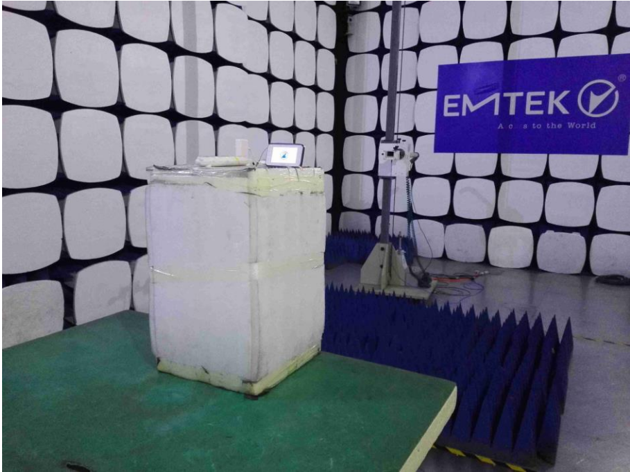
Photograph 3: Set-up for Radiated Spurious Emission, 18GHz - 26.5GHz
