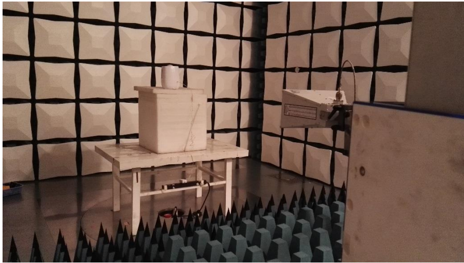
Photograph 3: Set-up for Radiated Spurious Emission, 1GHz ~ 26.5GHz
