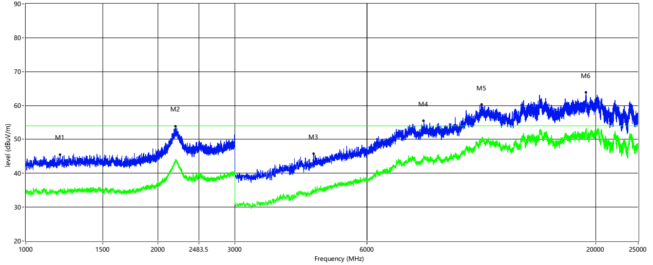
RE_FCC Test Case_FCC 15C 1GHz-25GHz
