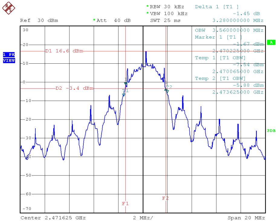
Figure 4– Result data graph shows 20 dB bandwidth, CF = 2.472GHz, BW = 3.56MHz
