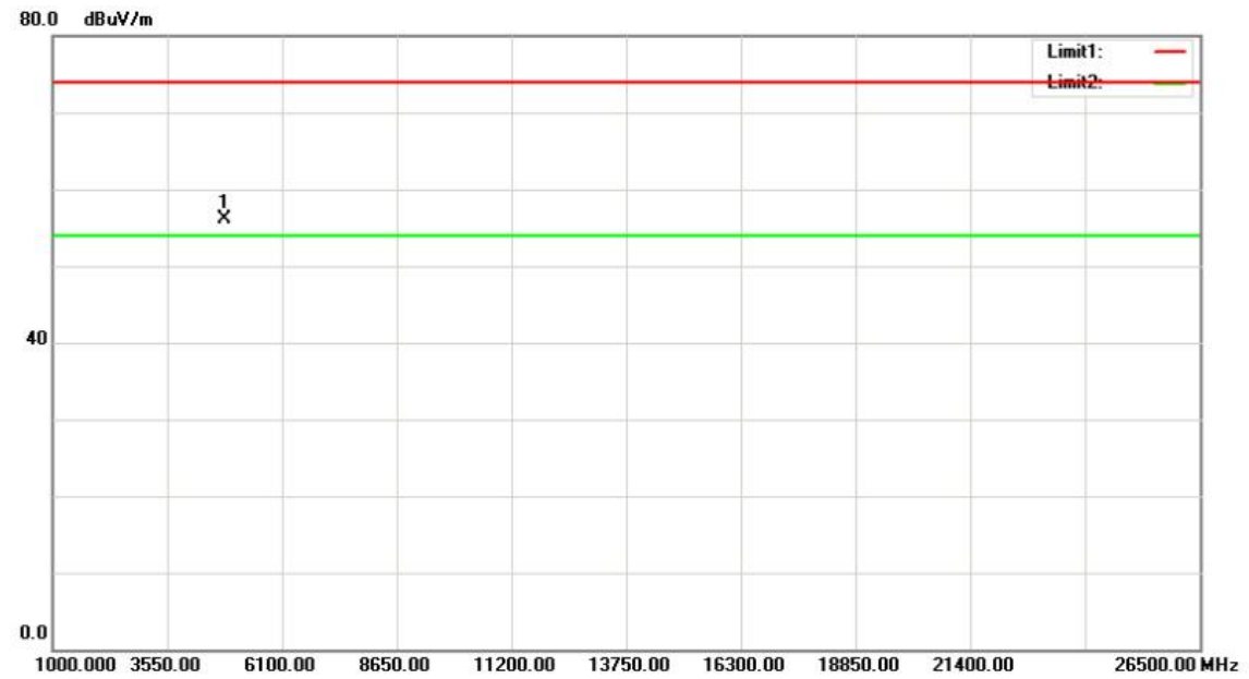
Figure 11 – Radiated emission data graph (Vertical polarization, 1GHz-26GHz) For Baby Unit
