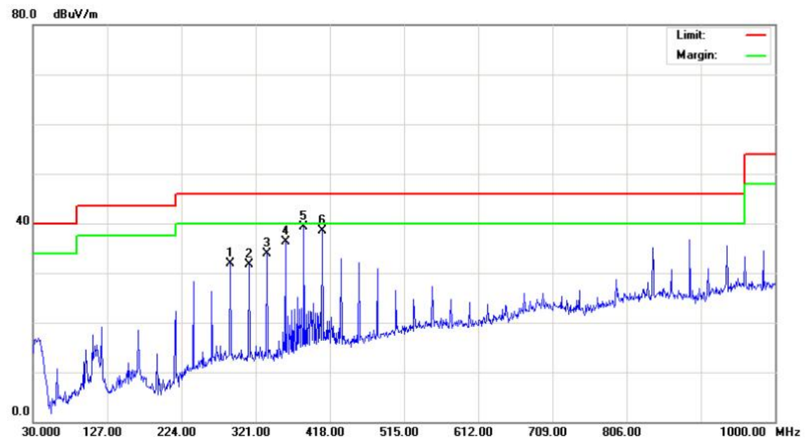
Figure 12 – Radiated emission data graph (Horizontal polarization, 30MHz-1GHz) For Baolijin Adaptor with Camera
