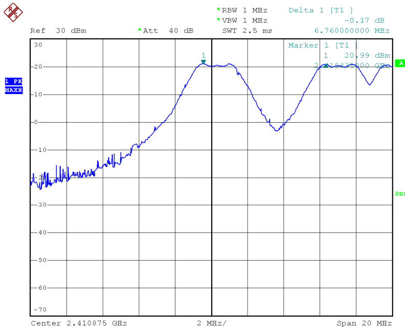
Figure 5 – Result data graph shows the channel separation:
