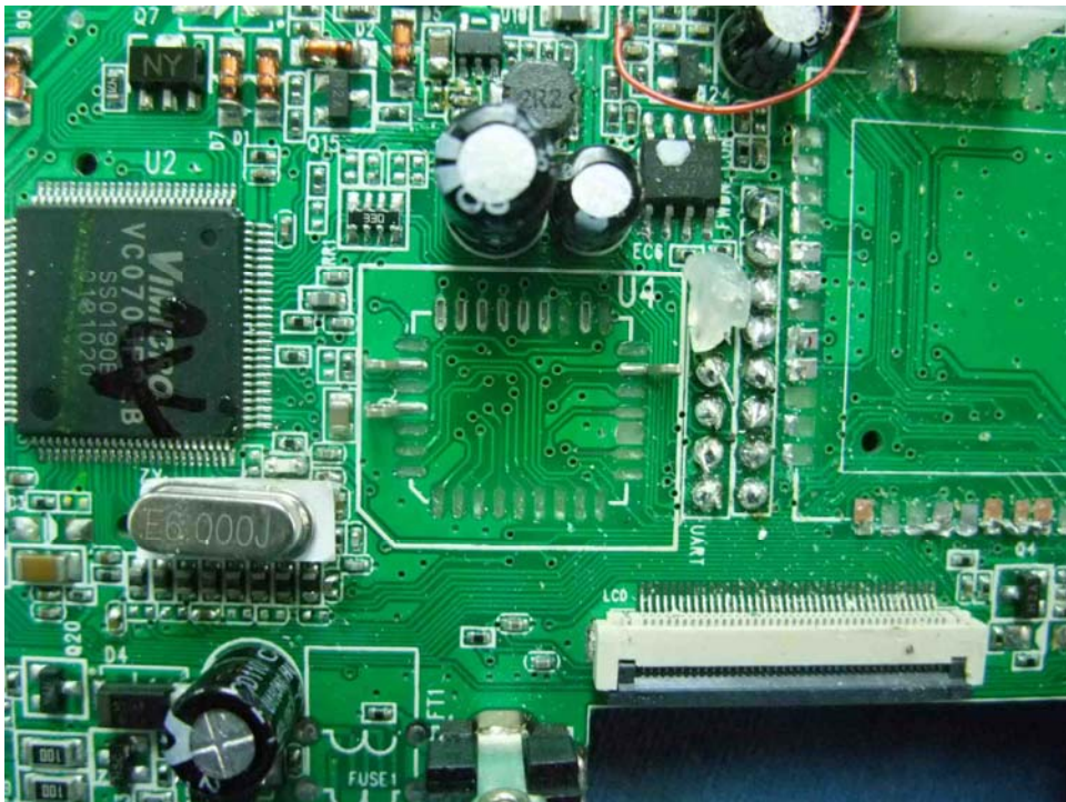
Parent Unit Main PCB comp side (View 3)
