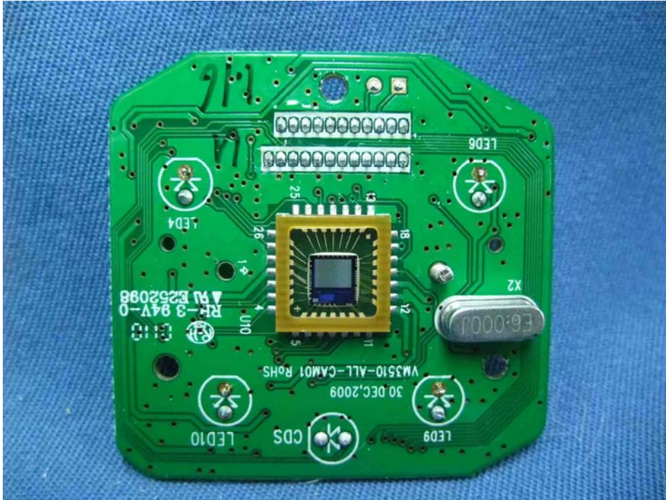
Camera Main PCB rear side (View 3)
