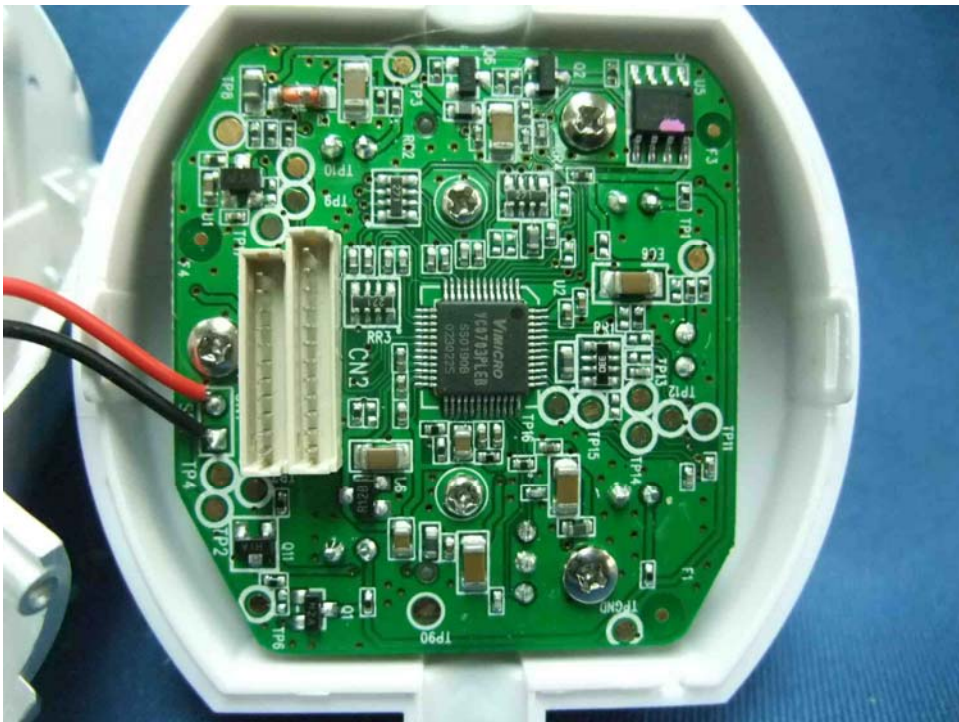
Camera Main PCB front side
