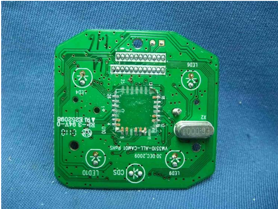
Camera Main PCB rear side (View 4)
