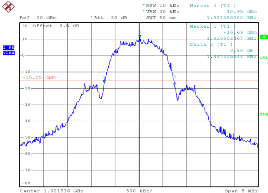
Parent unit, Lowest channel, Traffic carrier
