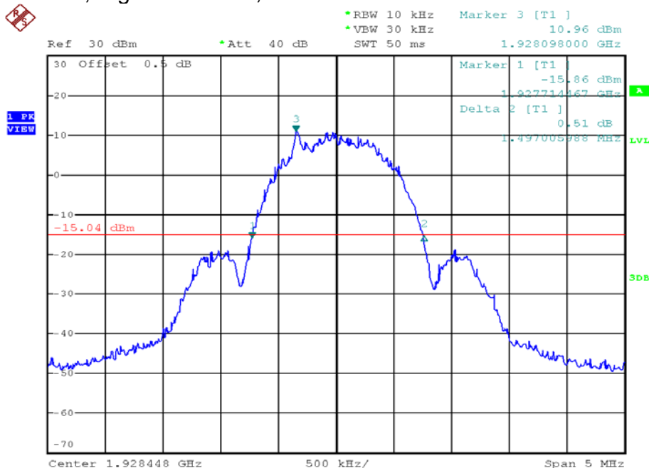
Parent unit, Highest channel, Traffic carrier
