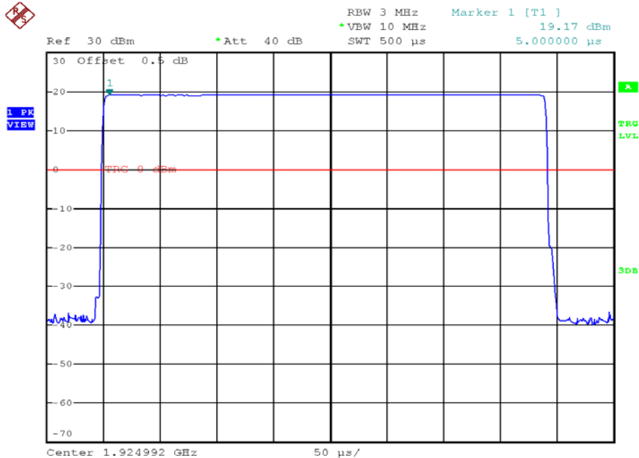
Parent unit, Middle channel, Traffic carrier
