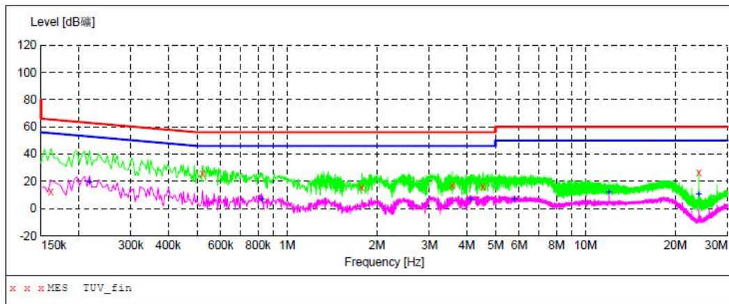
Phase N
