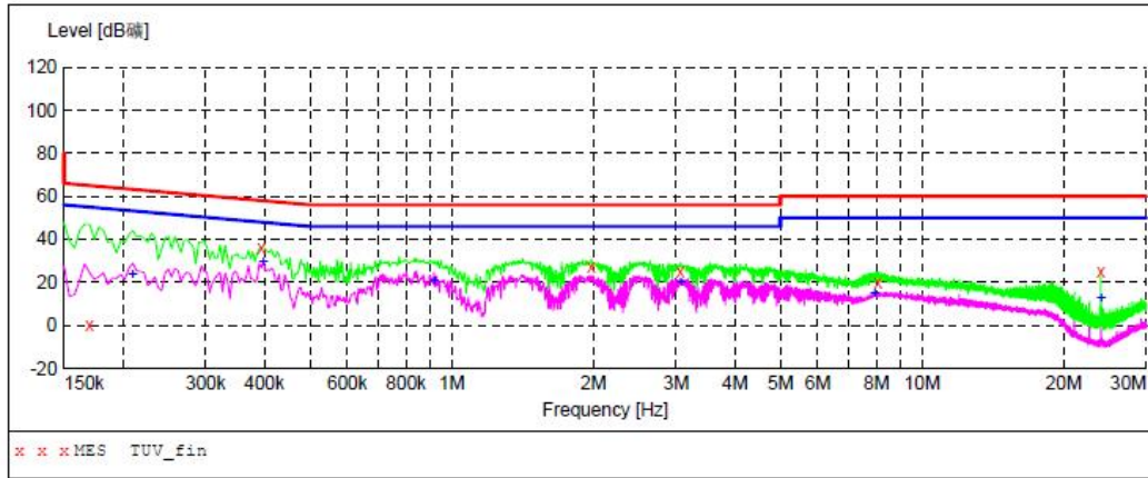
Phase L
