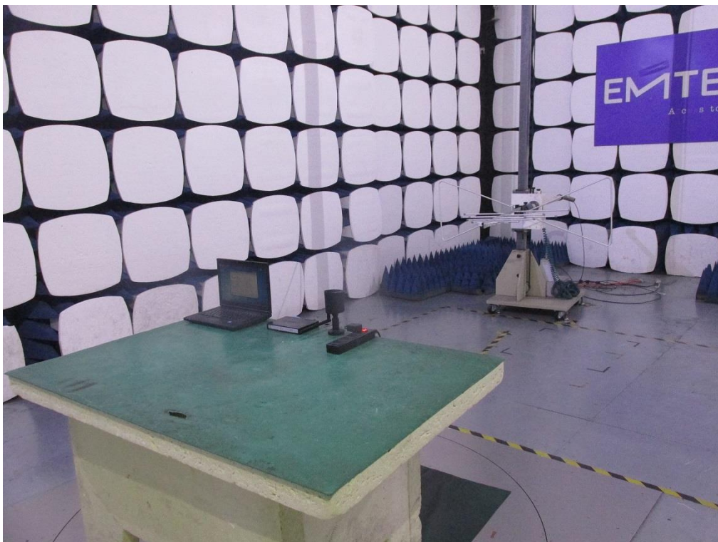
Photograph 4: Set-up for Radiated Emission, below 1GHz
