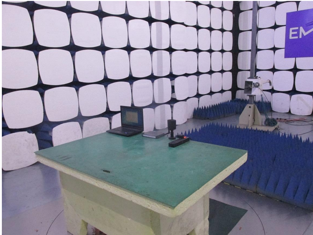
Photograph 5: Set-up for Radiated Emission, above 1GHz
