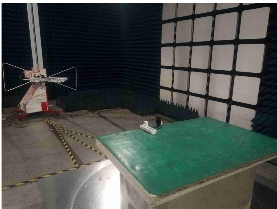
Photograph 6: Set-up for Radiated Emission, Below 1GHz
