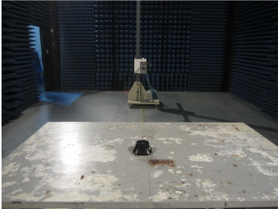
Figure 3 Setup for Radiated Emission (above 1GHz)
