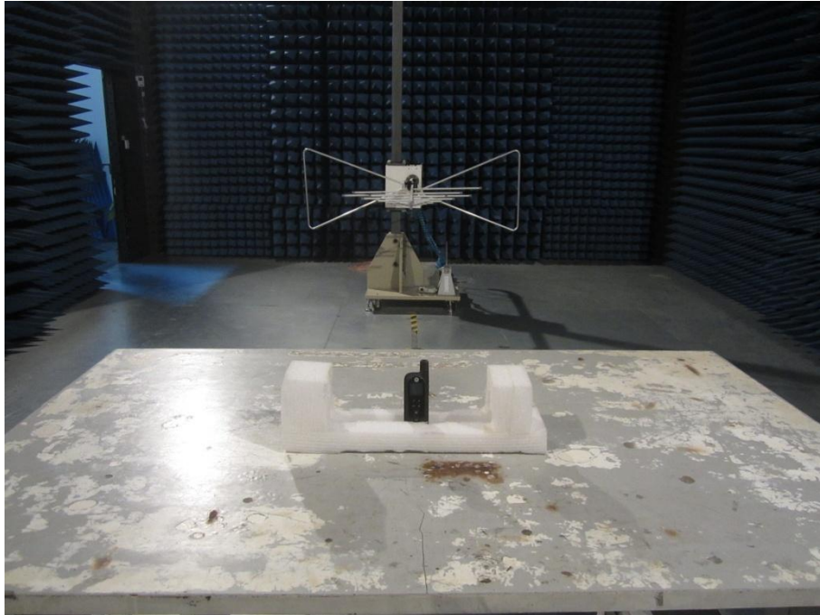
Figure 1 Setup for Radiated Emission(below 1GHz)
