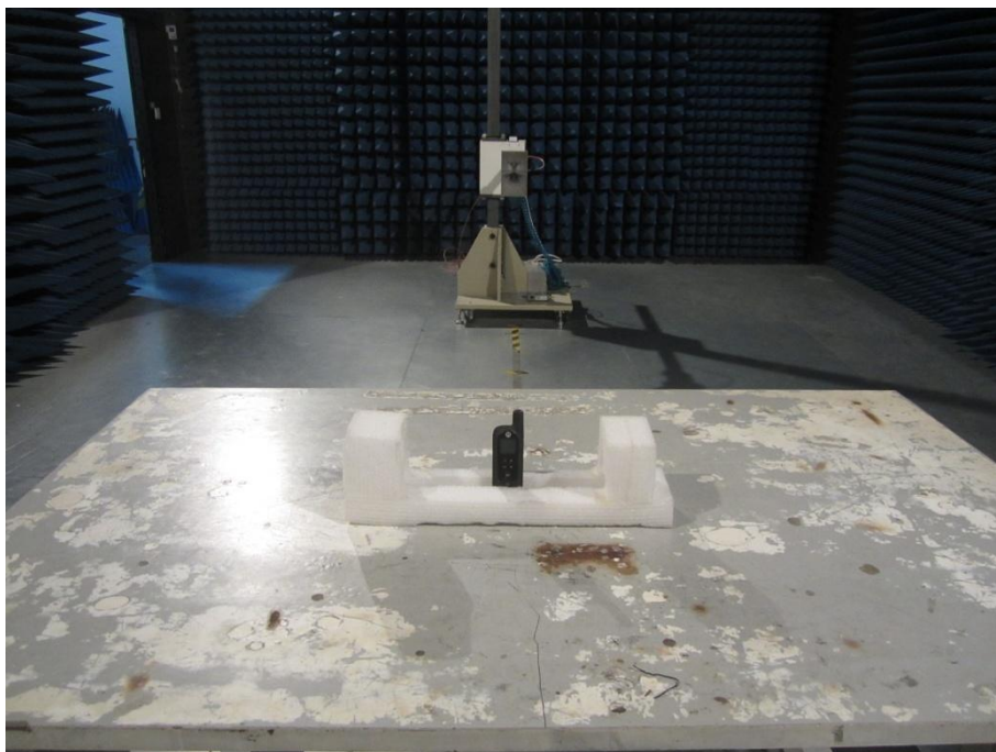
Figure 2 Setup for Radiated Emission (above 1GHz)
